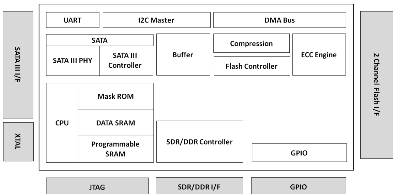
Figure 1-1 J320 2.5" SATA SSD Controller Block Diagram
