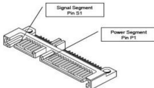
Figure 5-1 J320 2.5" SATA SSD Pin Assignment
